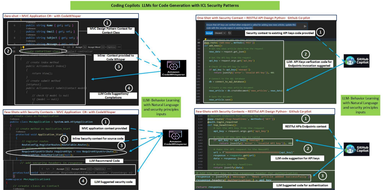
Figure 8: Coding Copilots dynamic contextual learning with ICL: Code Generation of GitHub Copilot and Code Whisperer
