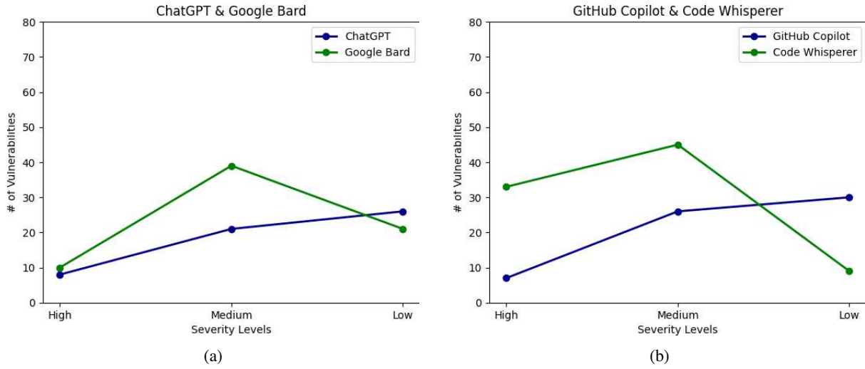
Figure 10: Security impact analysis from vulnerabilities
