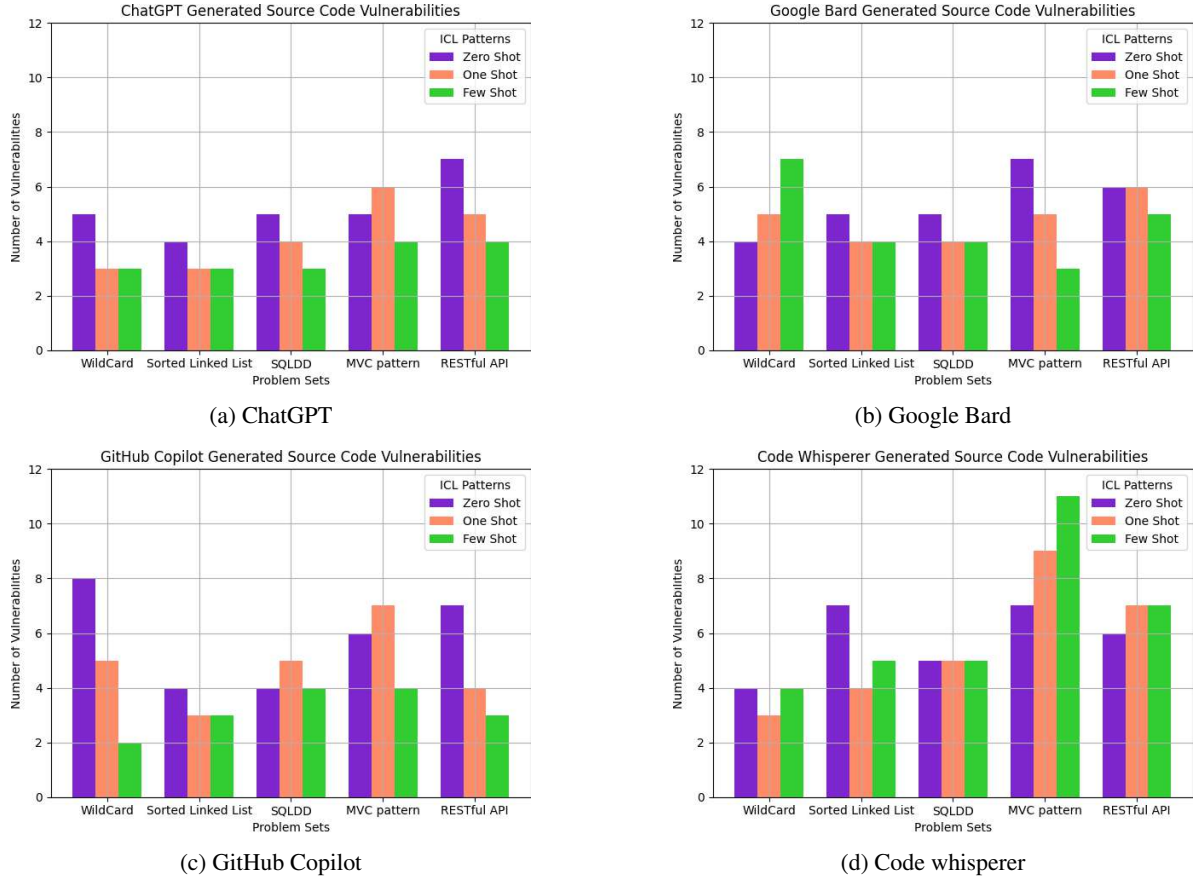
Figure 9: Comparison of Vulnerabilities Generated by ChatGPT, Google Bard, GitHub Copilot, and Code Whisperer
