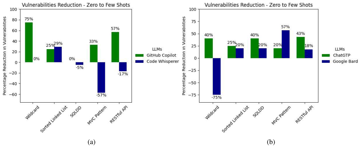
Figure 11: LLMs Code Vulnerability Reduction Analysis for LLMs- ICL security patterns
