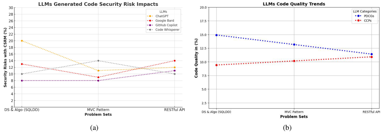
Figure 13: LLMs impact on security risks and code quality.
