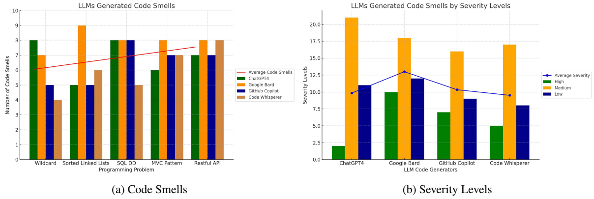
Figure 12: LLMs generated Code Smells and Risks
