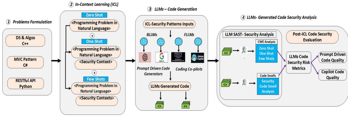
Figure 5: Large Language Models Code Evaluations Framework using ICL Security Patterns
