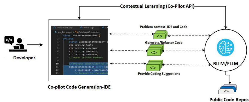
Figure 3: Coding CoPilots LLMs for Code Generation
