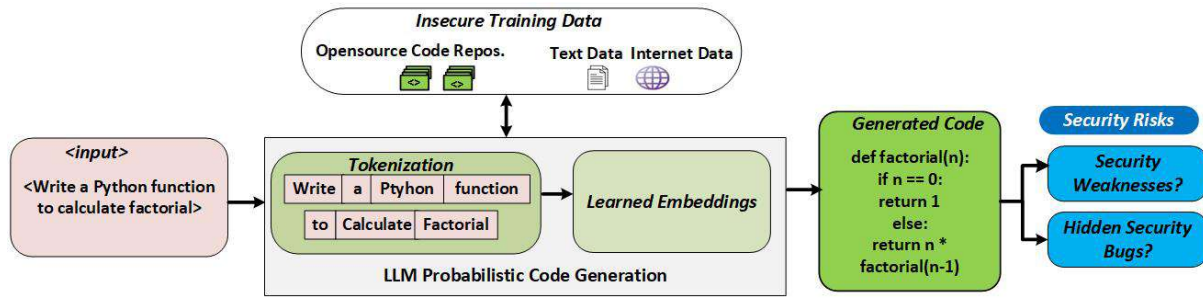
Figure 1: The LLM code generation process: simplified Transformer architecture for code generation with potential security risks
